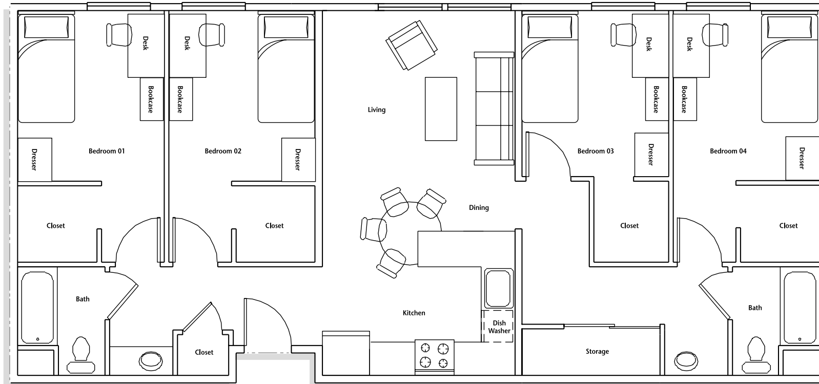
4 bedroom_floorplan_type a
